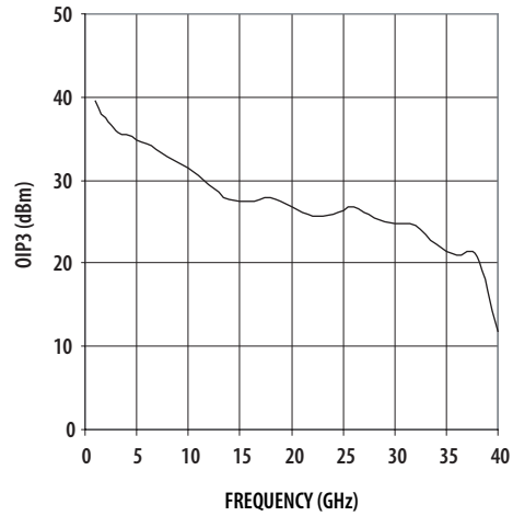
Figure 4. Output IP3.
