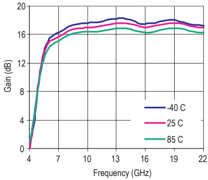
Figure 14. Gain and Temperature
