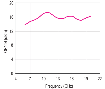
Figure 6. P1dB
