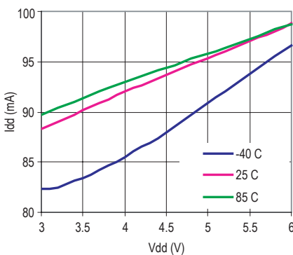
Figure 20. Idd vs. Vdd
