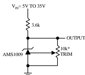
2.5V Reference
