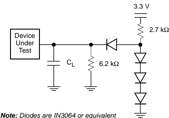
Figure 11. Test Setup
