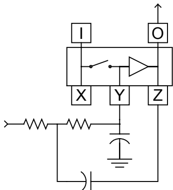
Figure 8. A 2 nd Order Sallen-Key Filter for Input Anti-Aliasing
