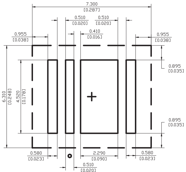
Figure 5: Recommended Minimum Pad Layout
