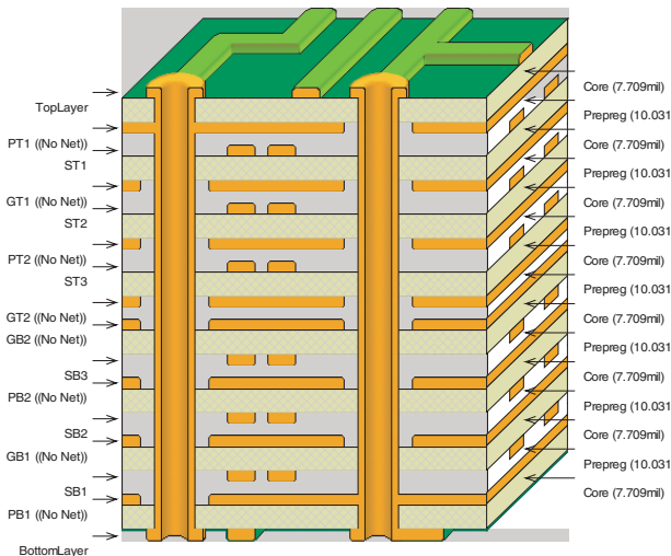
Figure 3: PCB Layer-Stack
