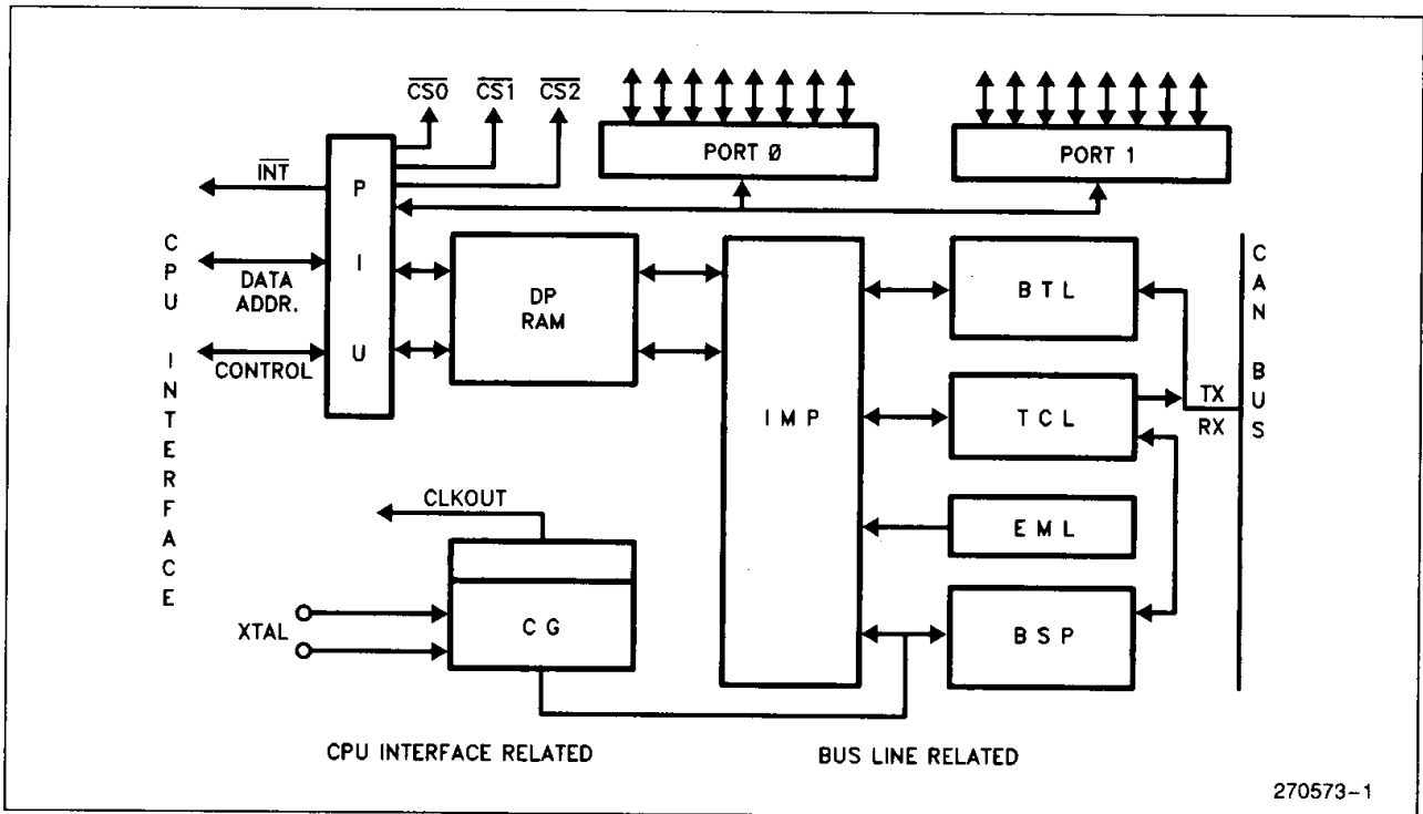
Figure 1. 82526 Block Diagram
