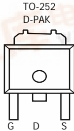
Top View Drain Connected to T_{oh}
