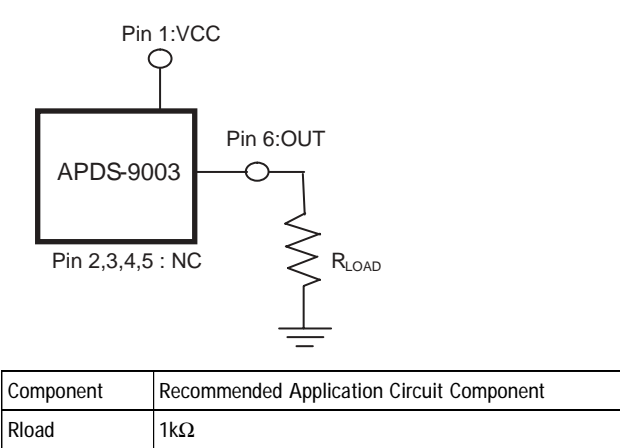
Figure 1: Typical application circuit for APDS-9003
