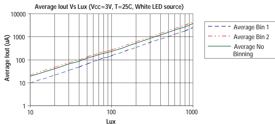
Average Iout Vs Lux (Vcc = 3V, T = 25C, White LED source)
