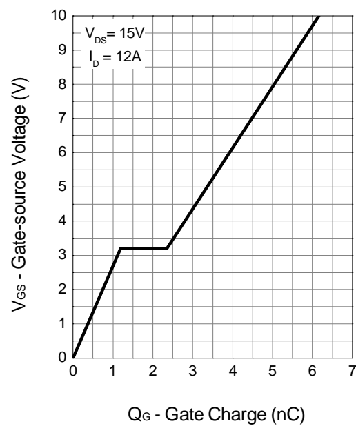
Gate Charge
