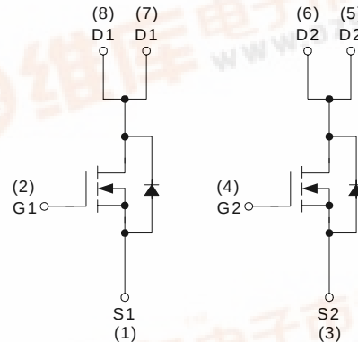
N-Channel MOSFET
