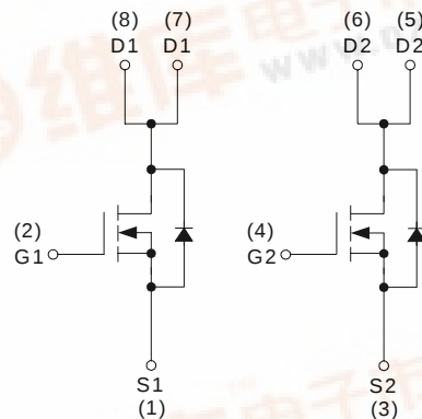
N-Channel MOSFET
