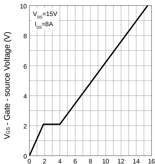
Gate Charge
