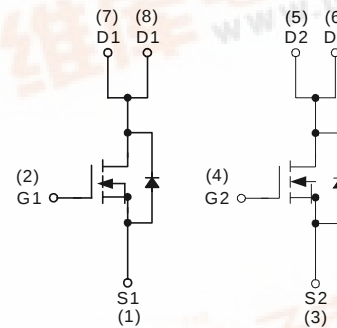
N-Channel MOSFET
