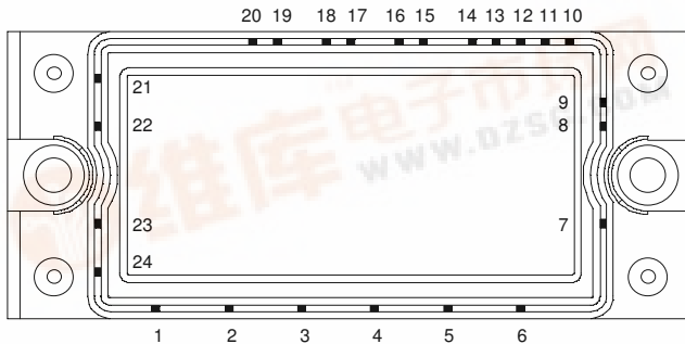
APTGS25X120RTP2: Without Brake (Pin 7 &amp; 14 not connected)
