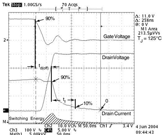
Figure 23, Turn-off Switching Waveforms and Definitions
