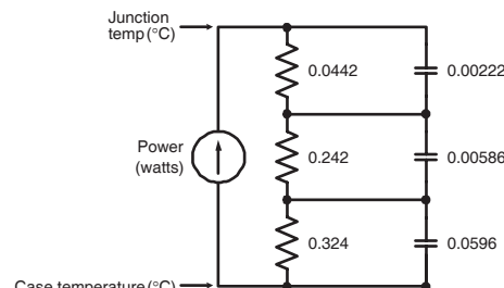
FIGURE 24a. MAXIMUM EFFECTIVE TRANSIENT THERMAL IMPEDANCE, JUNCTION-TO-CASE vs. PULSE DURATION RC MODEL
