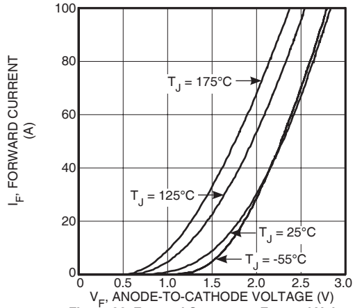
Figure 26. Forward Current vs. Forward Voltage
