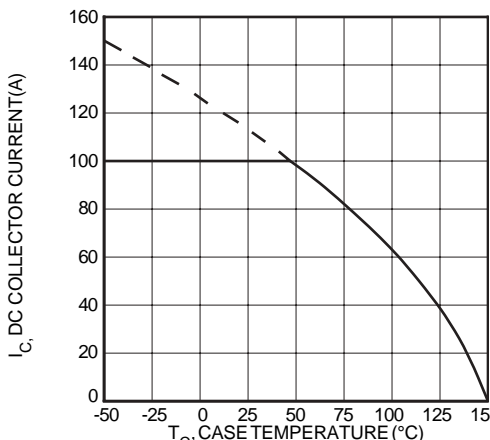
FIGURE 8, DC Collector Current vs Case Temperature
