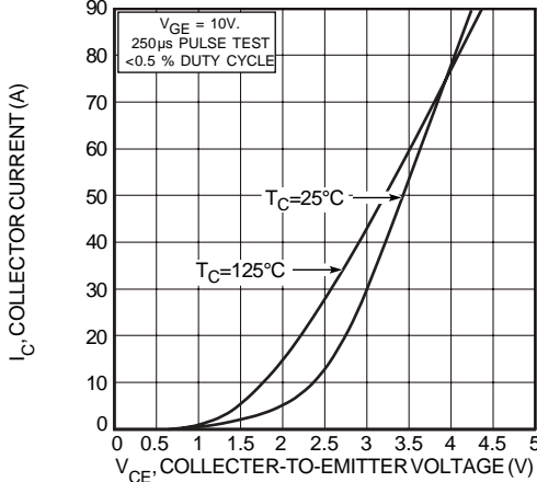
FIGURE 2, Output Characteristics ( V_{GE} = 10V )
