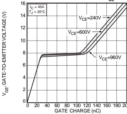
FIGURE 4, Gate Charge
