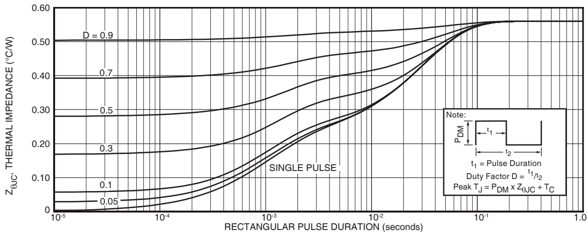
Figure 12. Maximum Effective Thermal Impedance Junction-to-Case vs Pulse Duration
