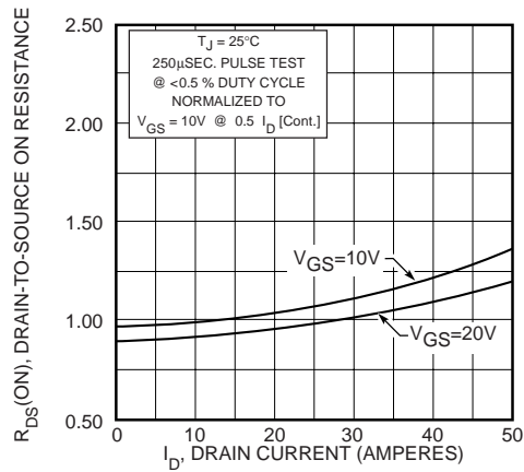
FIGURE 5, R_{DS}(\text{ON}) vs DRAIN CURRENT
