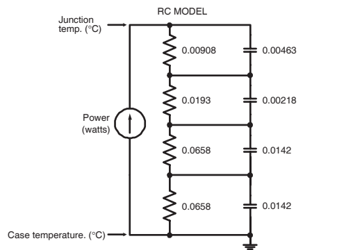
FIGURE 19b, TRANSIENT THERMAL IMPEDANCE MODEL
