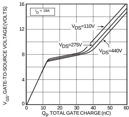
FIGURE 12, GATE CHARGE vs GATE-TO-SOURCE VOLTAGE
