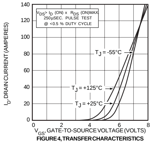
FIGURE 4, TRANSFER CHARACTERISTICS
