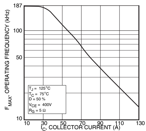
Figure 20, Operating Frequency vs Collector Current
