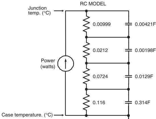
FIGURE 2, TRANSIENT THERMAL IMPEDANCE MODEL
