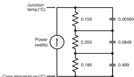
FIGURE 25a. MAXIMUM EFFECTIVE TRANSIENT THERMAL IMPEDANCE, JUNCTION-TO-CASE vs. PULSE DURATION RC MODEL
