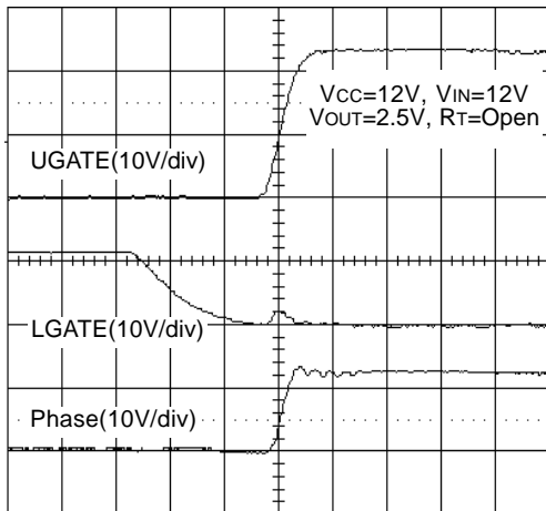
UGATE Rising
