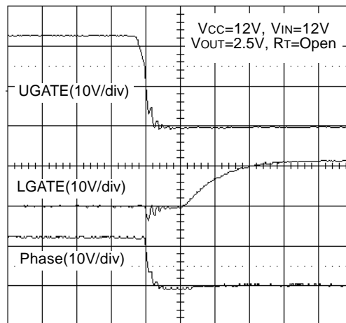
UGATE Falling
