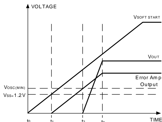
FIGURE1. SOFT-START INTERVAL
