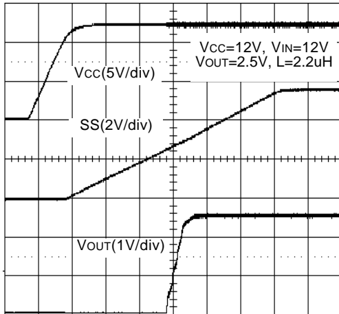
Power Up
