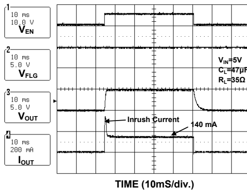
Turn-On/Turn-Off (AP1212H)
