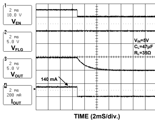
Turn-Off (AP1212H)
