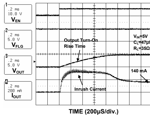
Turn-On (AP1212H)
