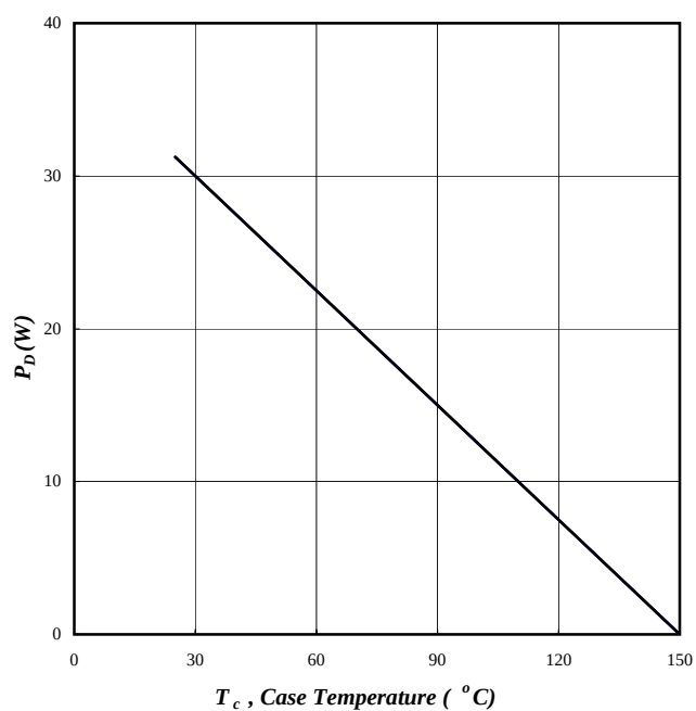
Fig 6. Typical Power Dissipation
