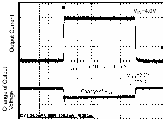
Figure 14. Load Transient
