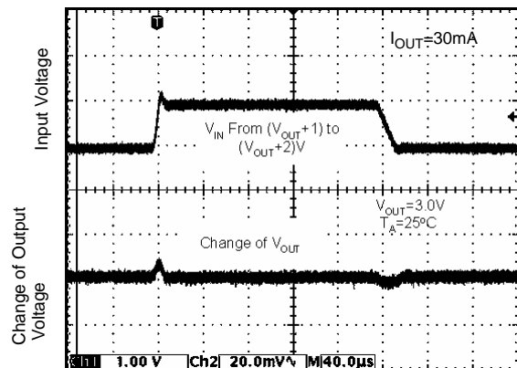
Figure 15. Line Transient
