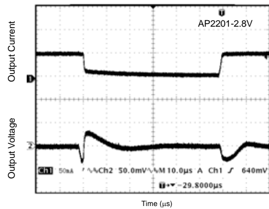
Figure 12. Load Transient (Conditions: V_{IN}=3.8V , C_{BYN}=680pF , V_{EN}=2V , I_{OUT}=5mA to 50mA , C_L=2.2µF )
