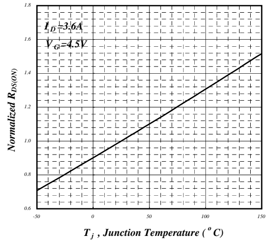
Fig 4. Normalized On-Resistance
