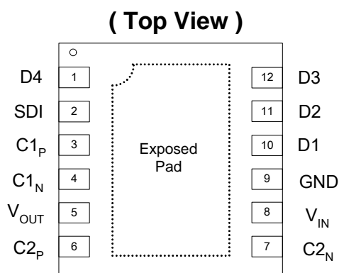
DFN3030-12
