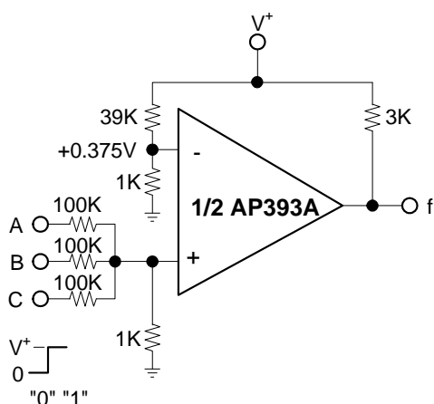
AND Gate
