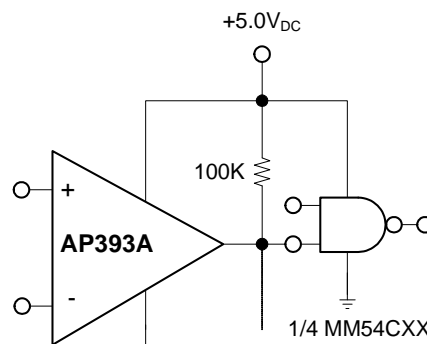
Driving CMOS
