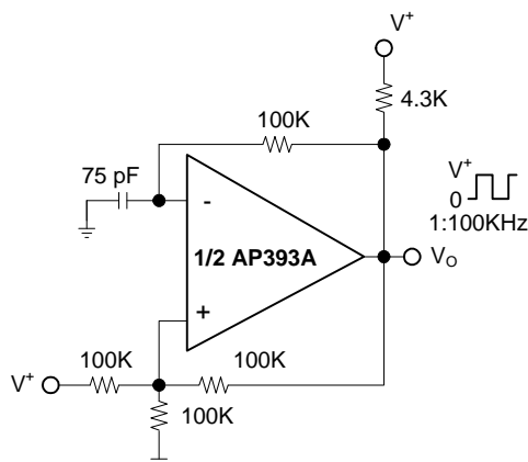
Squarewave Oscillator
