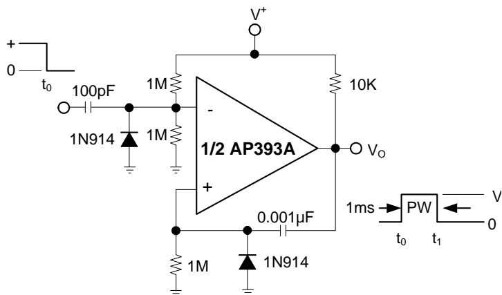
One-Shot Multivibrator
