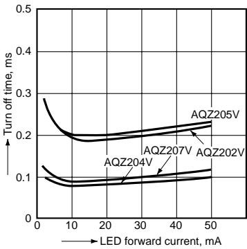
12. LED forward current vs. turn off time characteristics
