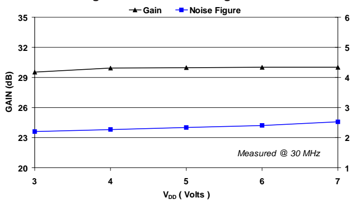
Figure 7: Gain & Noise Figure vs V_{DD}
