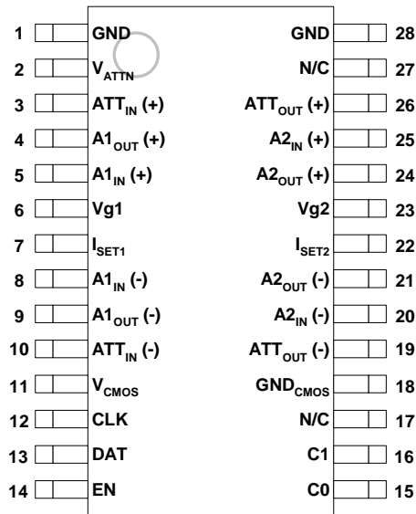
Figure 3: Pin Out
