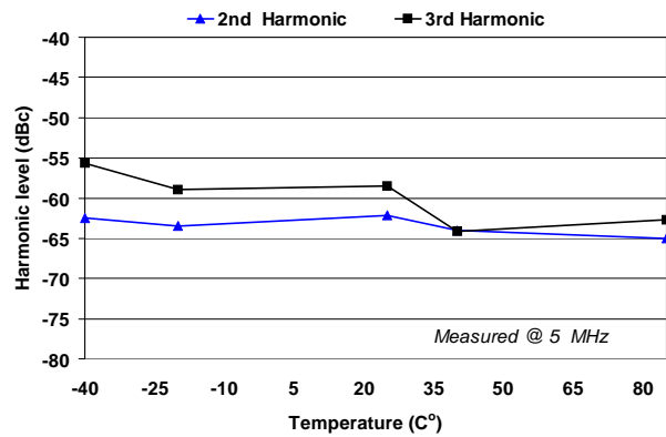
Figure 11: Harmonic Distortion vs Temperature P_{OUT} = 58\text{dBmV}
