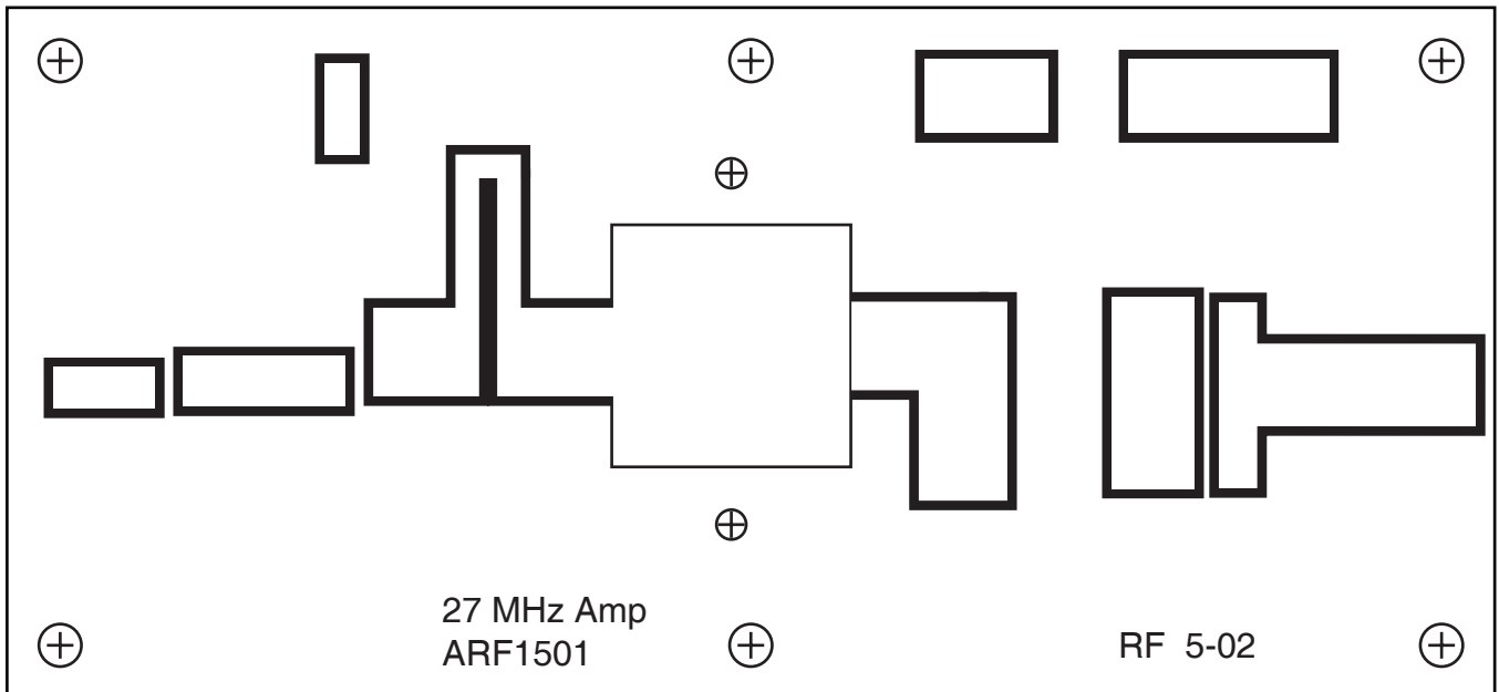
1:1 pcb artwork
