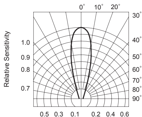
FIGURE 5. SENSITIVITY DIAGRAM
