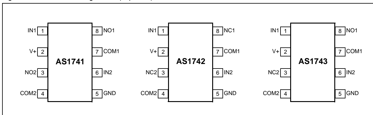
Figure 11. SOT23 Pin Assignments (Top View)
