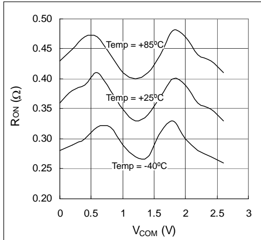
Figure 4. R_{ON} vs. V_{COM} and Temperature; V_{DD} = 2.7V
