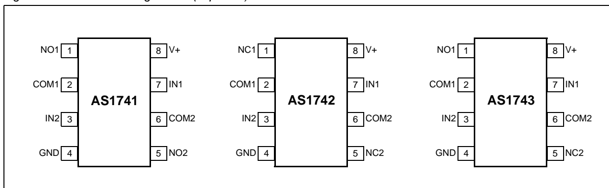
Figure 10. MSOP Pin Assignments (Top View)
