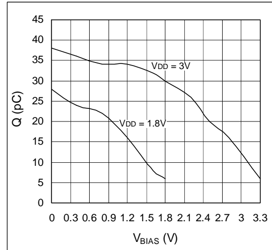
Figure 3. Charge Injection vs. Output Voltage; MSOP
