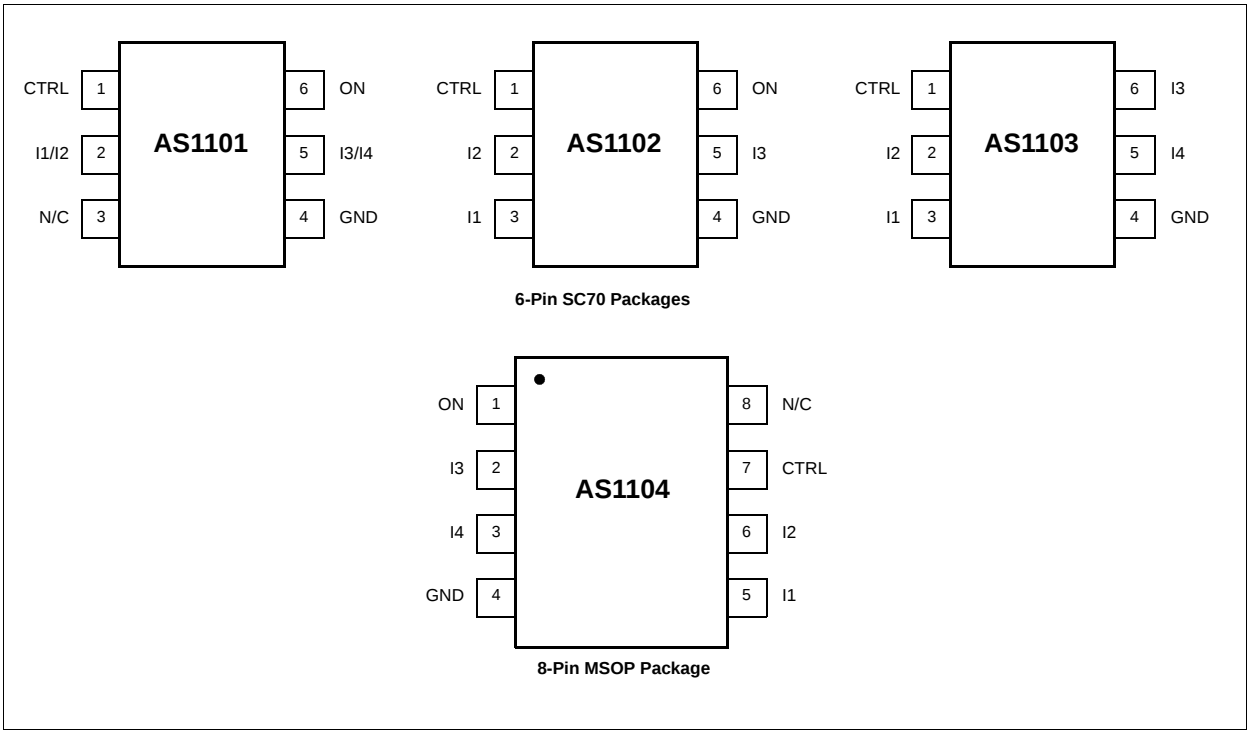
Figure 6. Pin Assignment – (Top View)
