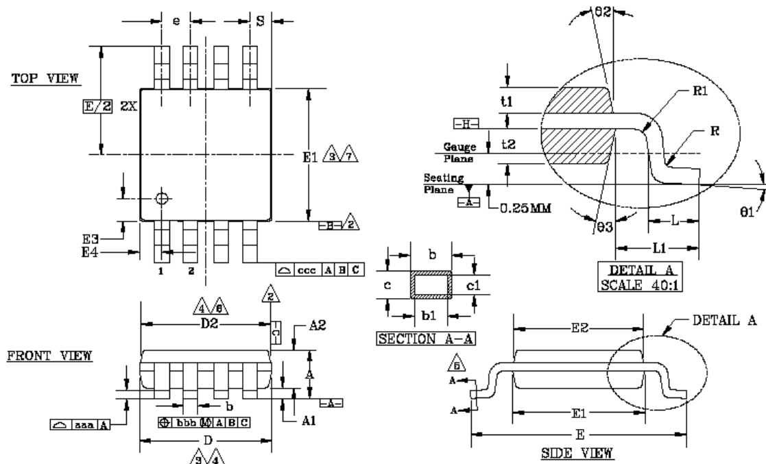
Figure 8. MSOP-8 Package
