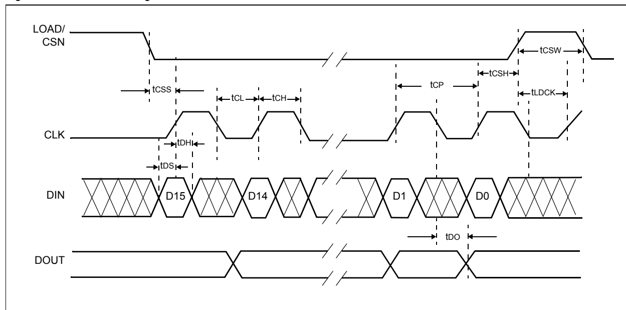
Figure 11. Interface Timing
