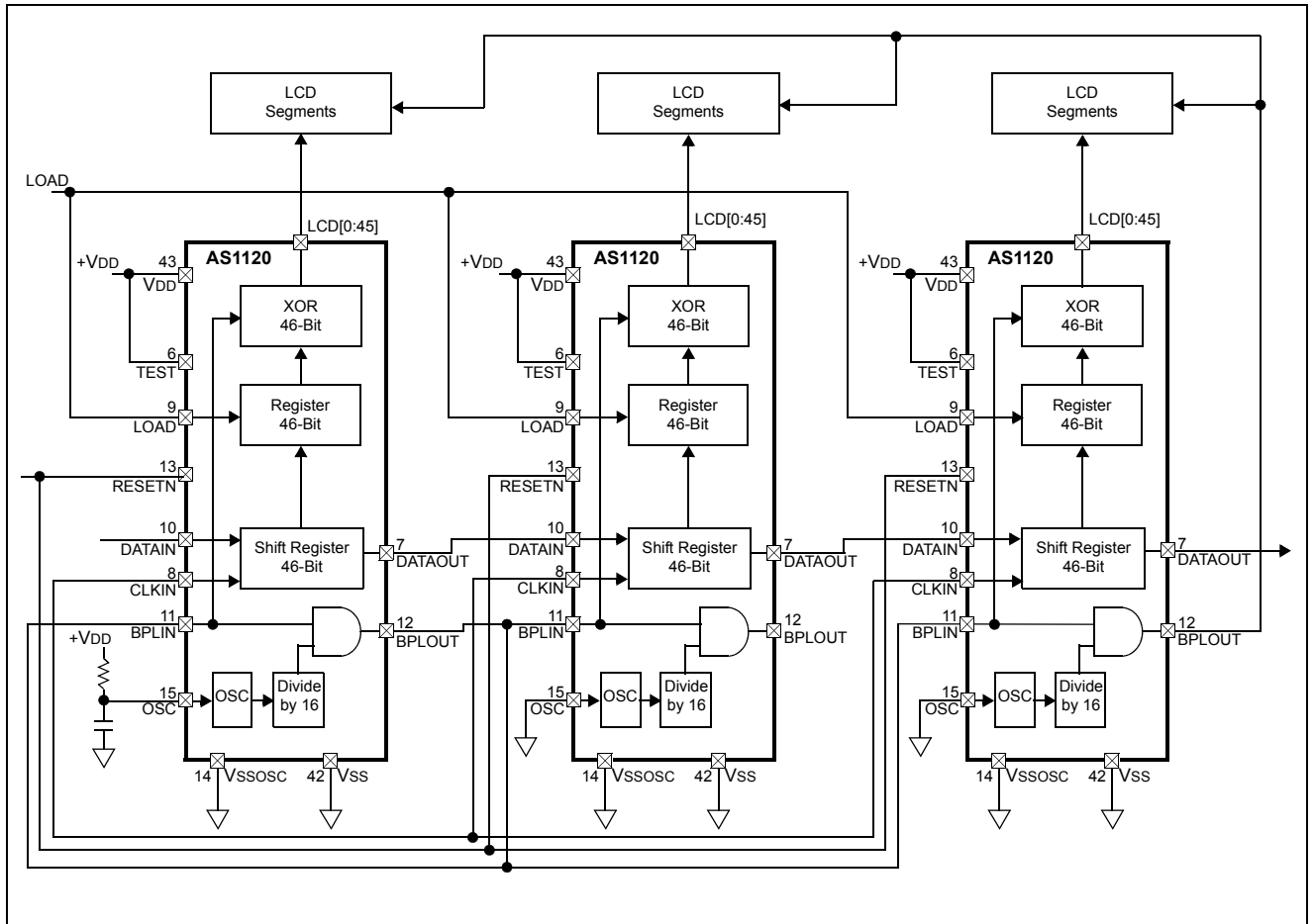
Figure 7. Cascaded Configuration
