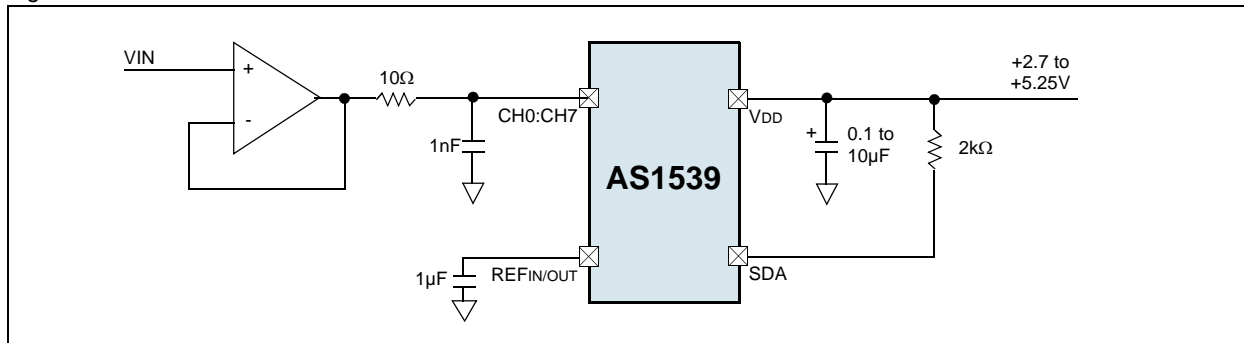
Figure 23. Reference circuit
