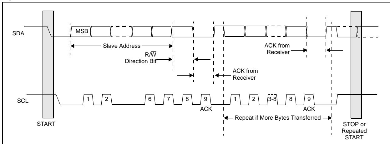
Figure 24. Bus Protocol
