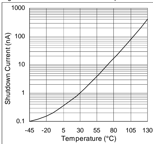
Figure 8. Shutdown Current vs. Temperature
