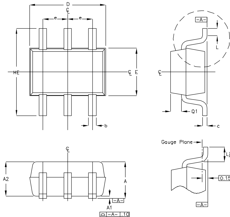
Figure 28. SC70-6 Package
