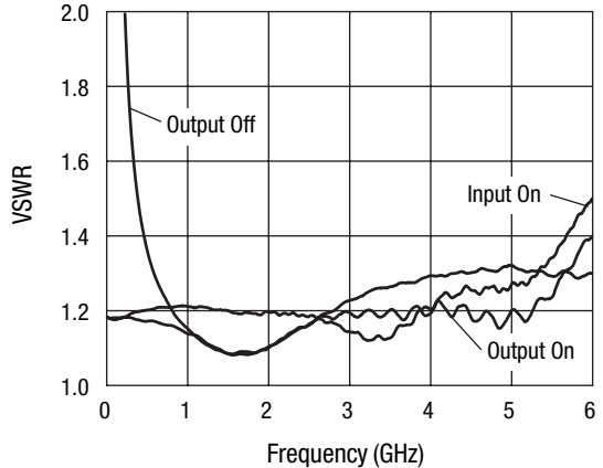
VSWR, 85 °C V DD = 5 V, V CTL = 0/5 V
