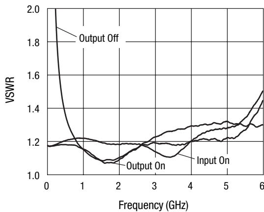
VSWR, 25 °C V DD = 5 V, V CTL = 0/5 V
