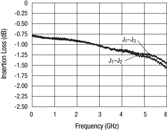
Insertion Loss, 85 °C V DD = 5 V, V CTL = 0/5 V
