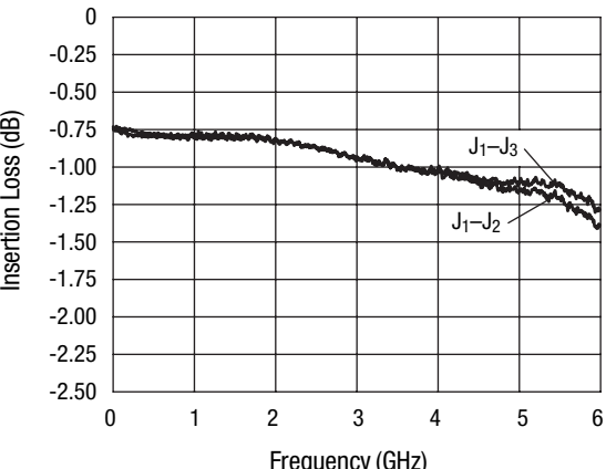
Insertion Loss, -40 °C V DD = 5 V, V = 0/5 V
