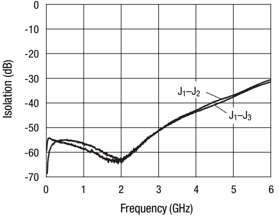
Isolation, 85 °C V DD = 5 V, V CTL = 0/5 V
