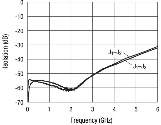
Isolation, -40 °C V DD = 5 V, V CTL = 0/5 V
