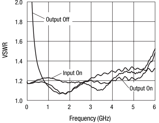
VSWR, -40 °C V DD = 5 V, V CTL = 0/5 V
