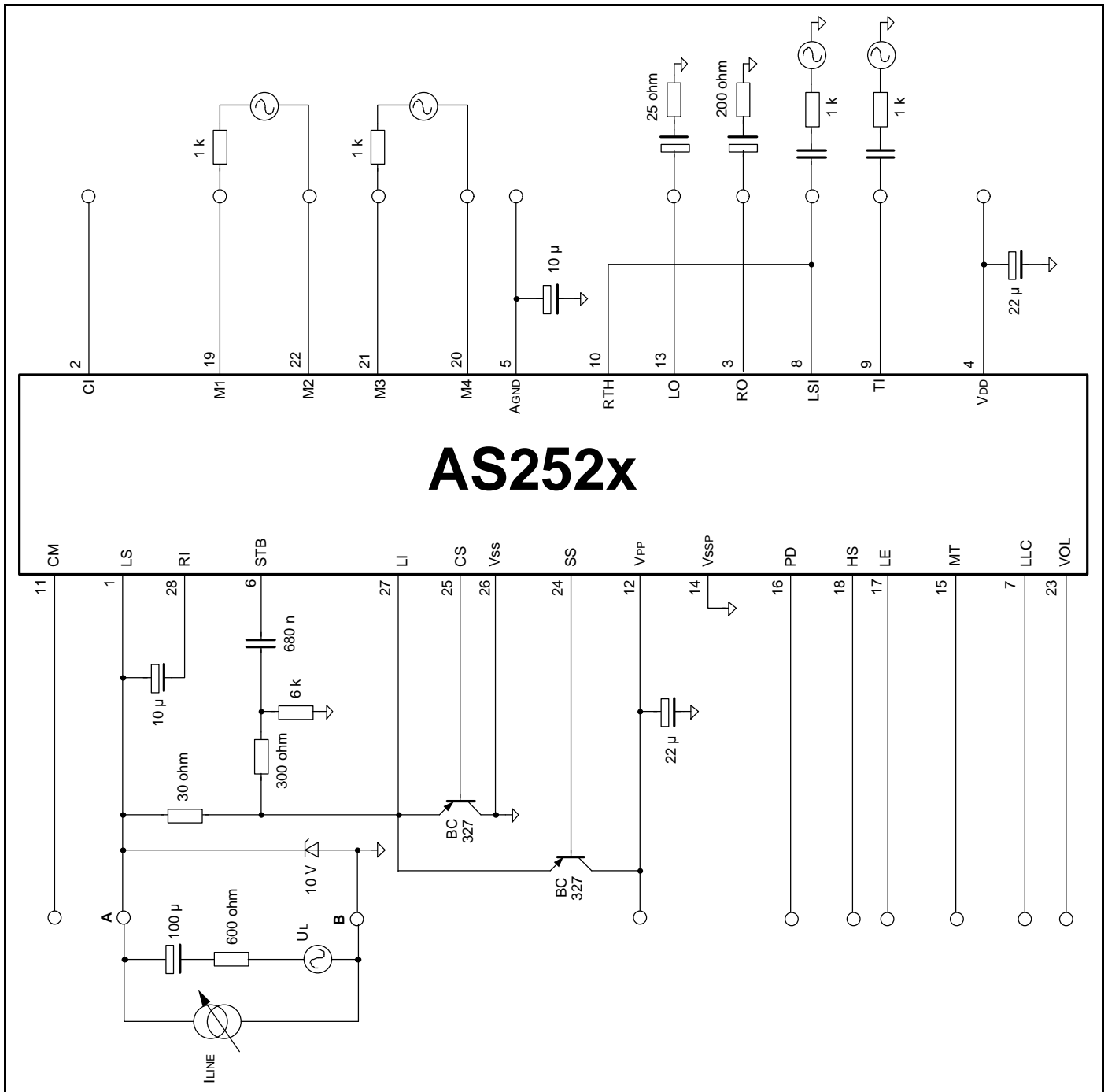
Figure 8: Test Circuit
