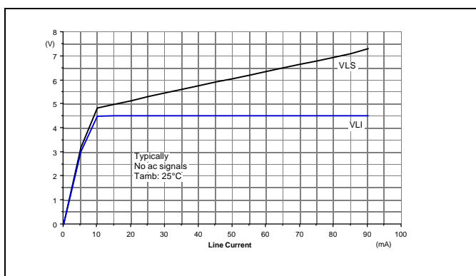
Figure 3: DC Mask
