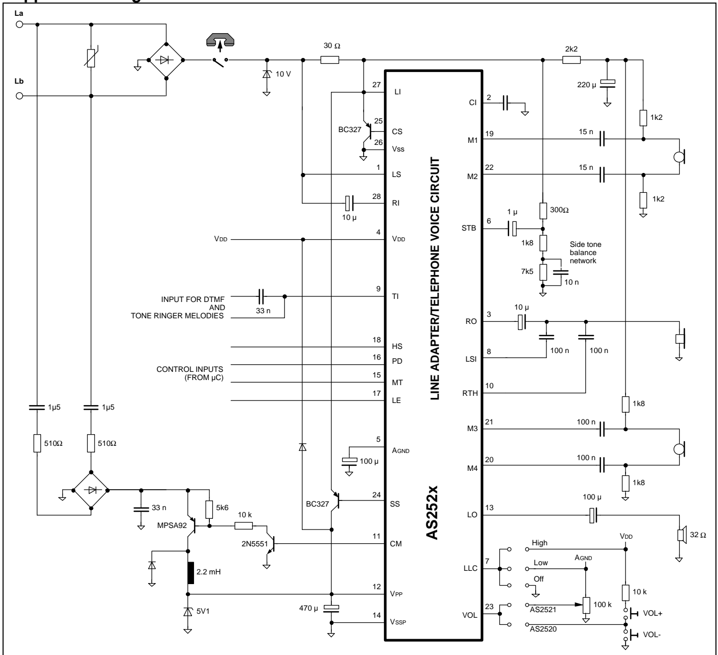
Figure 9: Application Diagramme
