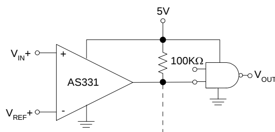
Figure 22. Driving CMOS
