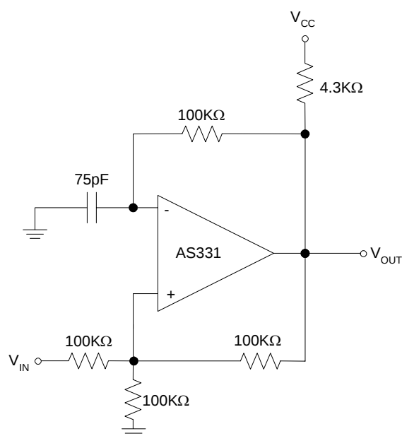
Figure 24. Squarewave Oscillator
