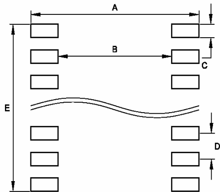
Figure 19. PCB Footprint
