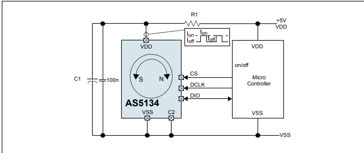
Figure 15. Low/Mid Power Mode Connection
