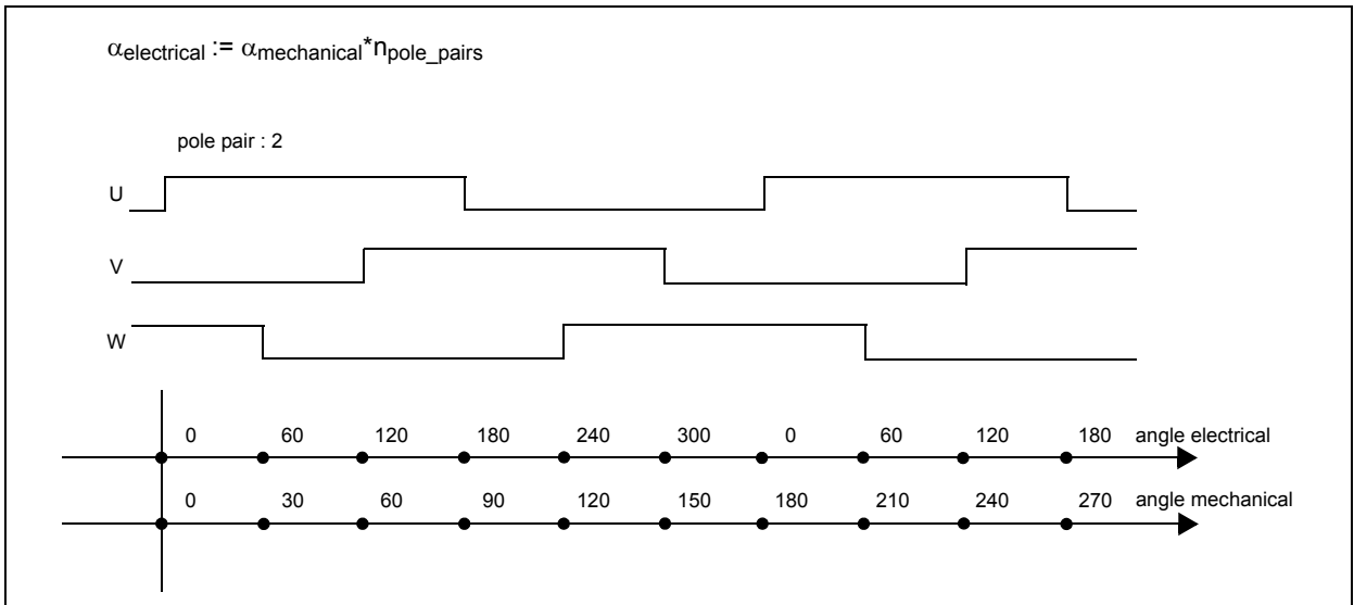
Figure 11. Commutation Mode
