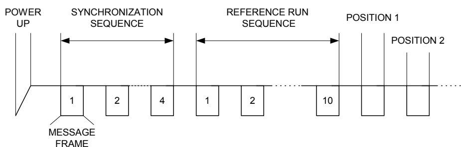
Figure 3-7. Necessary Commands after Power-up
