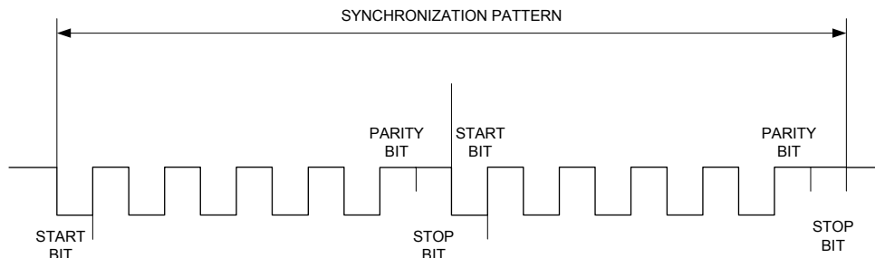
Figure 3-4. Synchronization Sequence
