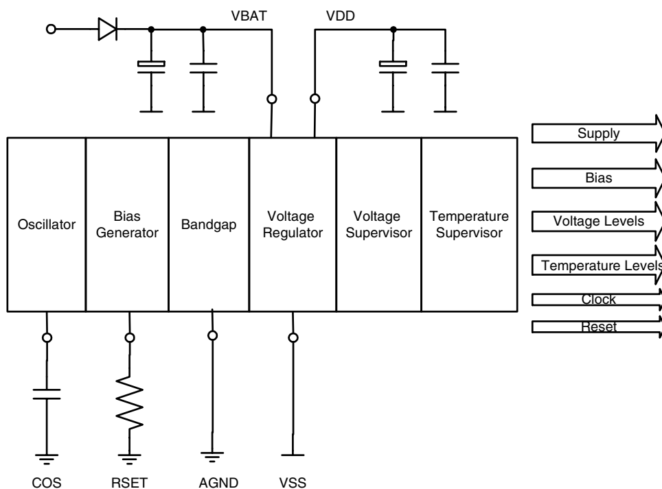
Figure 3-1. Analog Blocks
