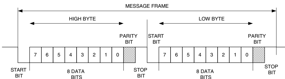
Figure 3-6. Command Bits
