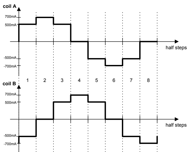
Figure 3-10. Compensated Halfstep Operation
