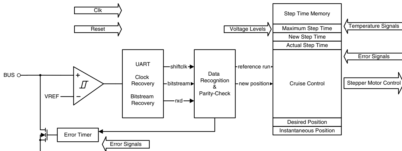
Figure 3-2. Digital Blocks
