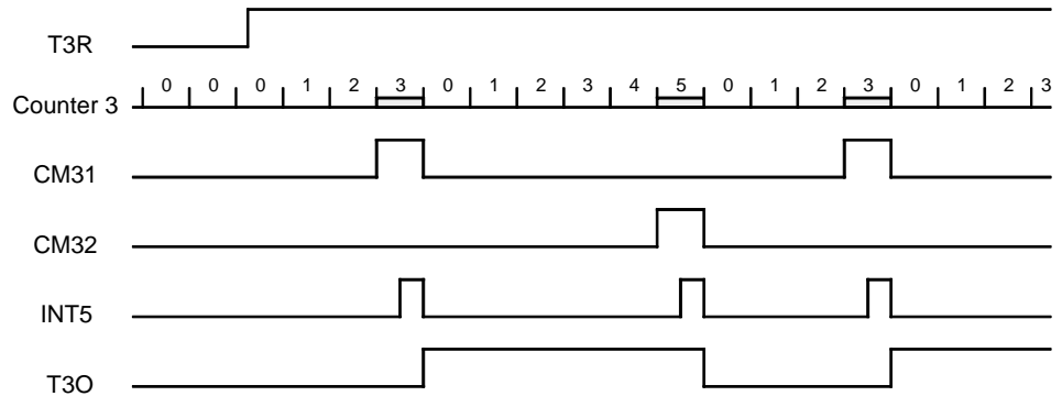
Figure 53. Counter Reset with Each Compare Match
