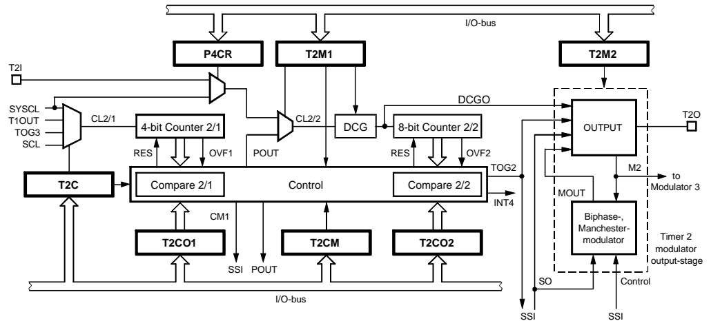
Figure 37. Timer 2
