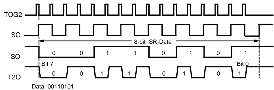
Figure 47. Biphase Modulation
