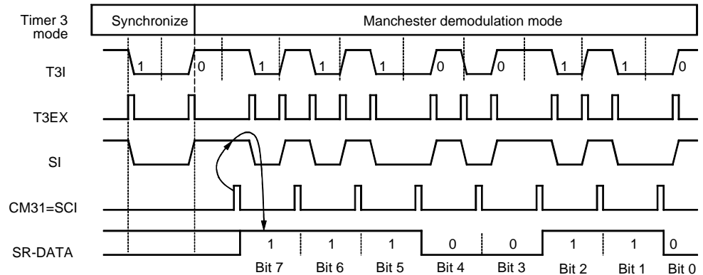
Figure 84. Manchester Demodulation
