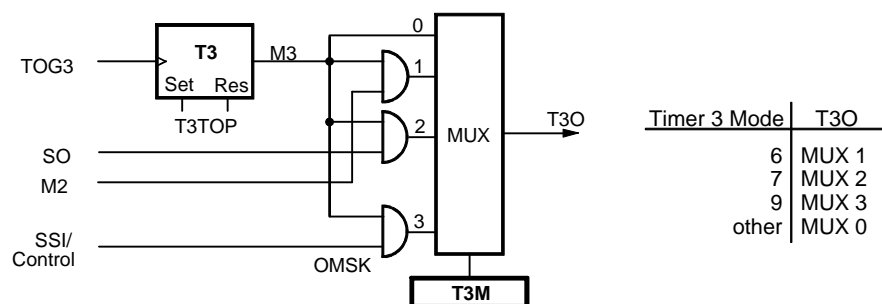
Figure 63. Modulator 3
