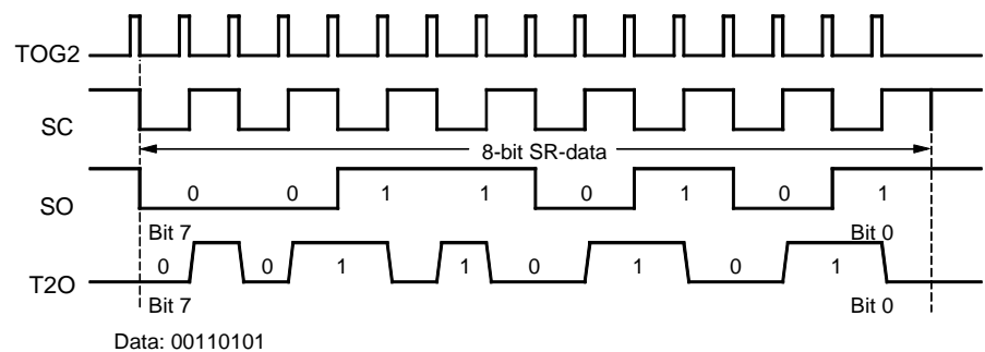
Figure 78. Manchester Modulation 1
