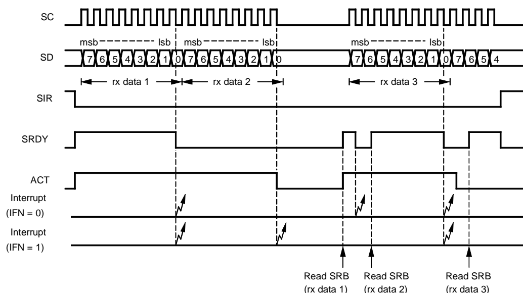
Figure 68. Example of 8-bit Synchronous Receive Operation
