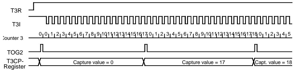
Figure 87. Frequency Measurement
