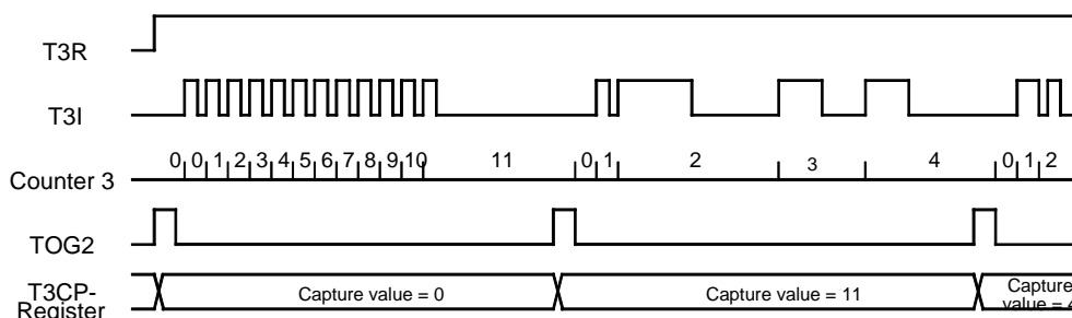
Figure 57. Event Counter with Time Gate
