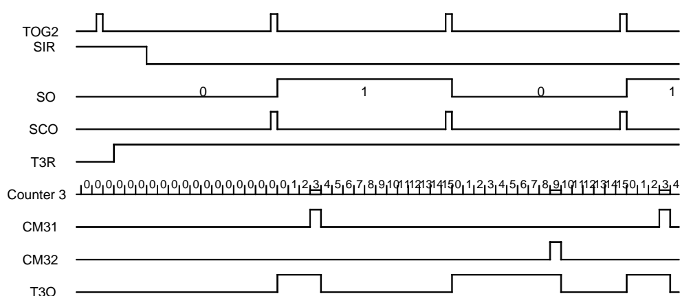
Figure 83. Pulse-width Modulation
