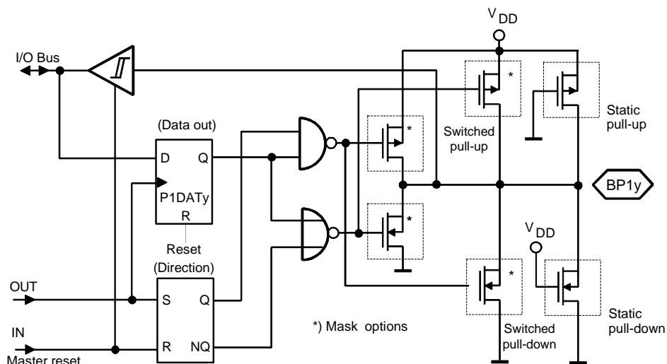
Figure 29. B-idirectional Port 1
