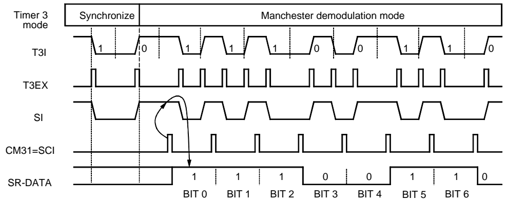
Figure 60. Manchester Demodulation
