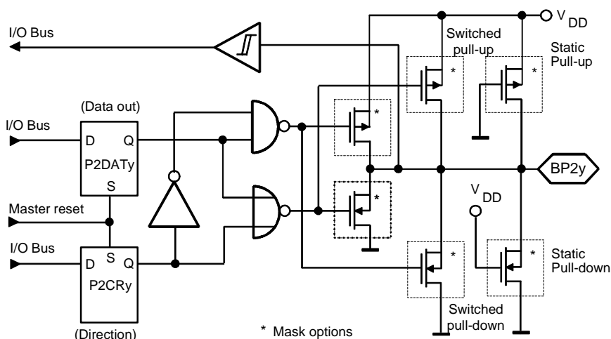
Figure 30. Bi-directional Port 2
