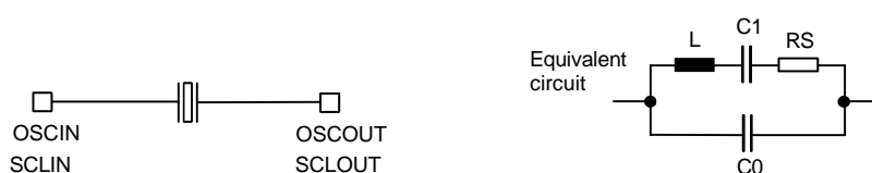
Figure 96. Crystal Equivalent Circuit
