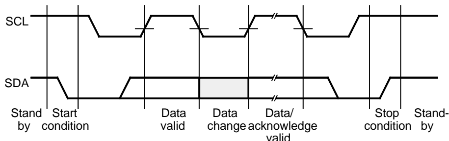
Figure 95. MCL Protocol
