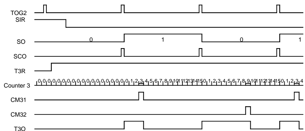
Figure 59. Pulse-width Modulation
