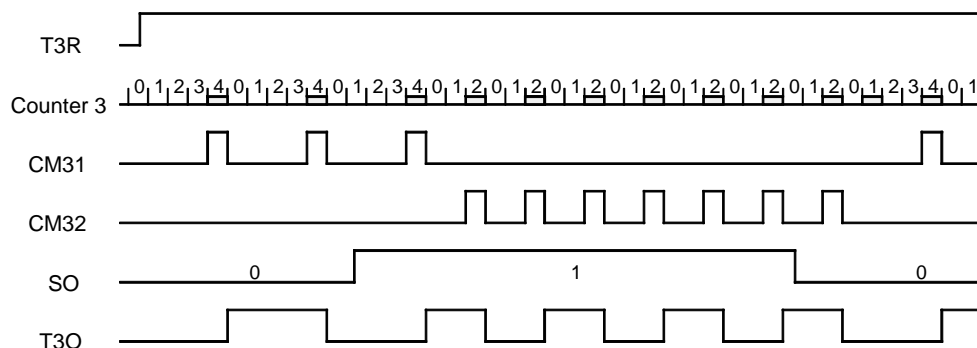
Figure 92. FSK Modulation
