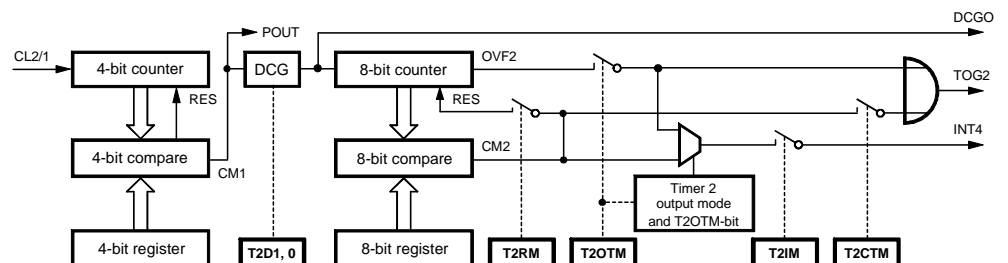
Figure 39. 8-bit Compare Counter
