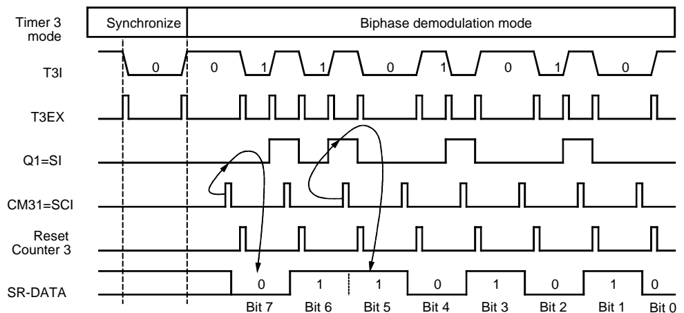
Figure 85. Biphase Demodulation
