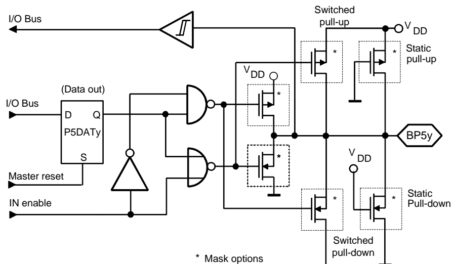
Figure 31. Bi-directional Port 5
