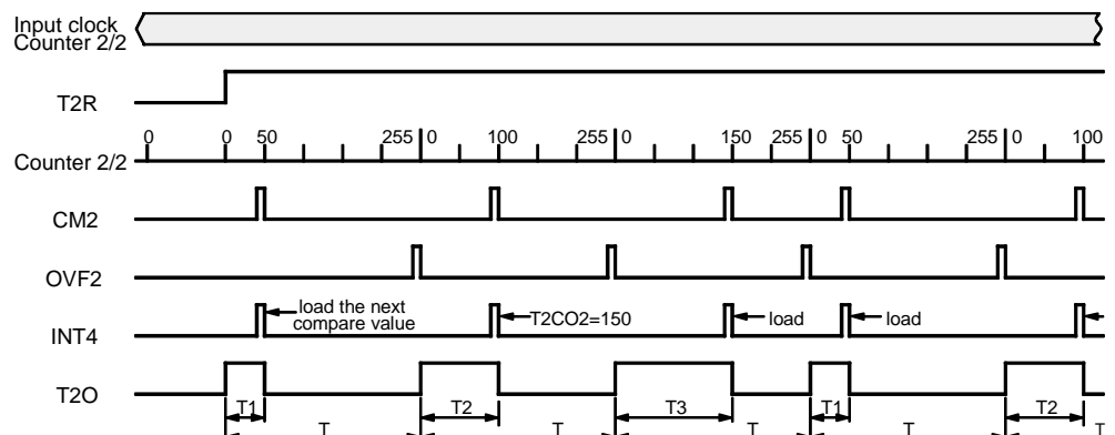
Figure 49. PWM Modulation
